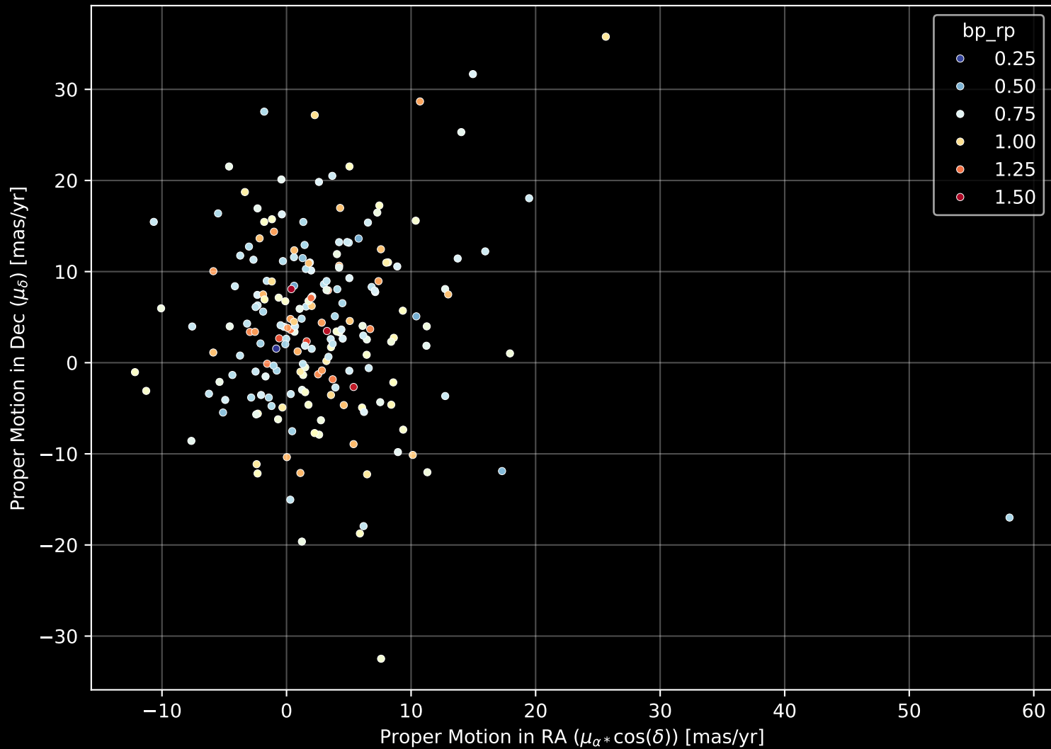
GALAH DR4 Field: [659] Proper Motion Diagram (n= 201)
