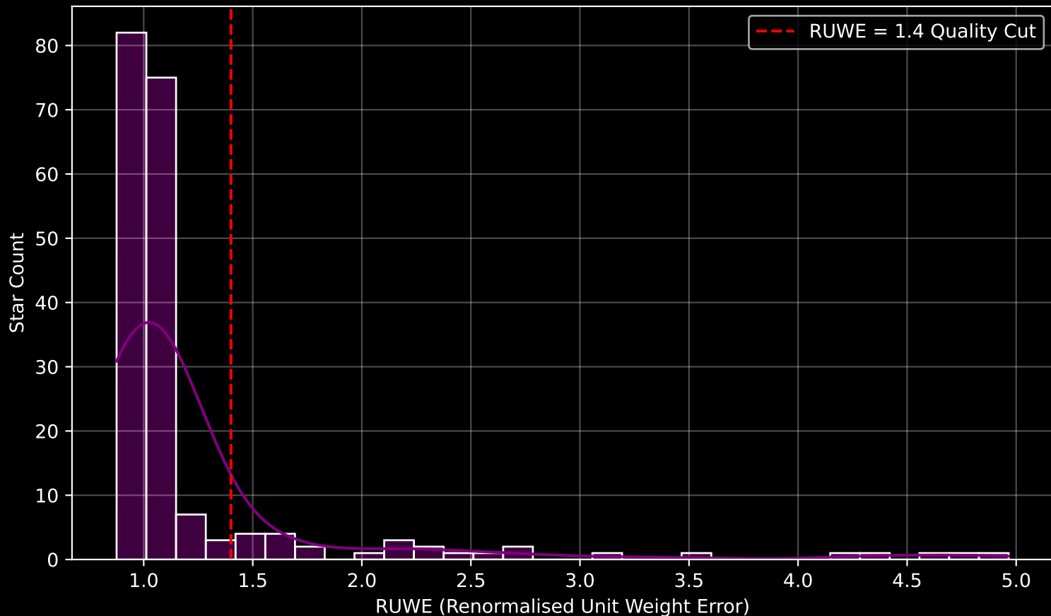
GALAH DR4 Field [659] RUWE Distribution (n= 194)
