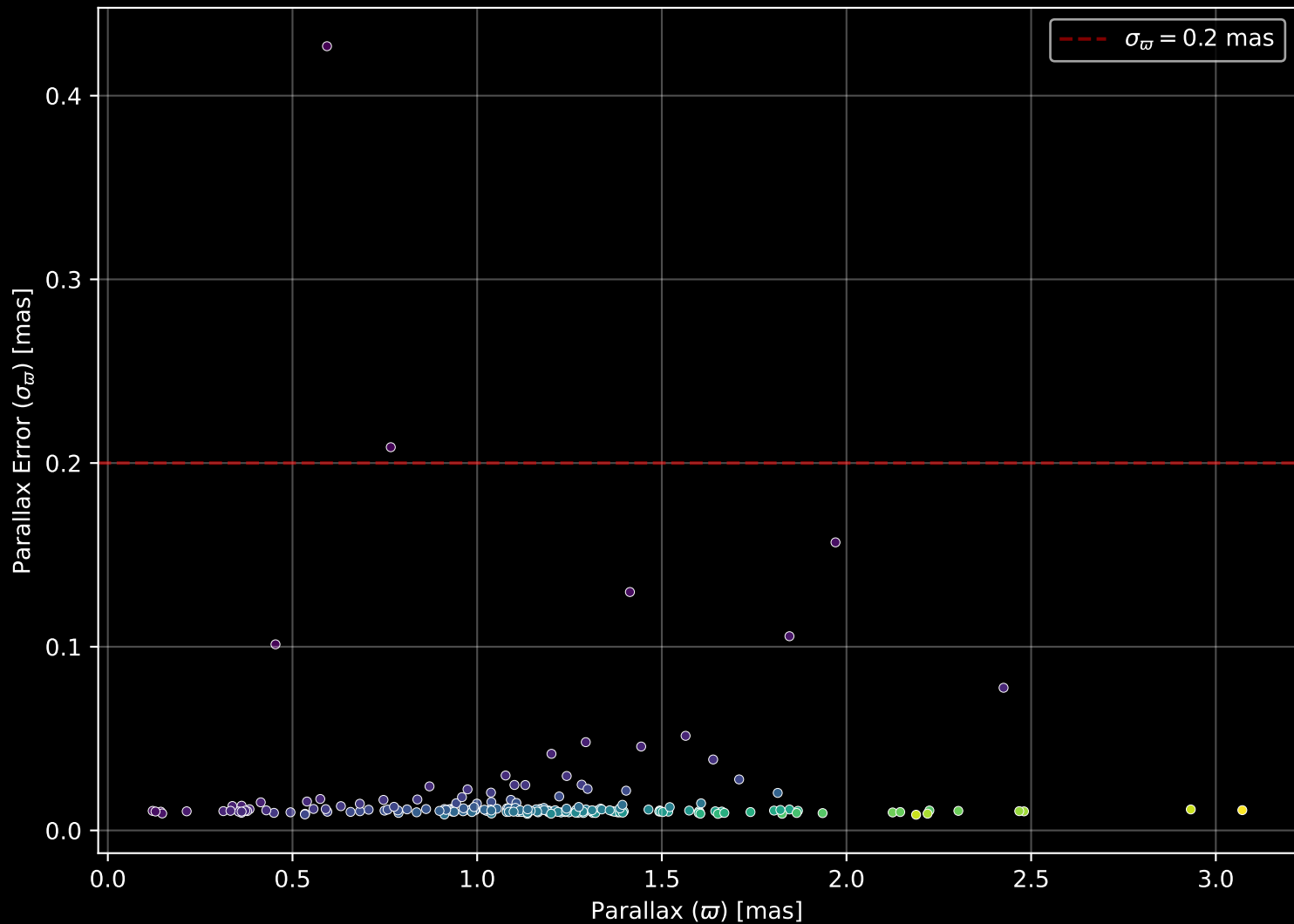
GALAH DR4 Field: [659] Parallax Quality (n= 201)
