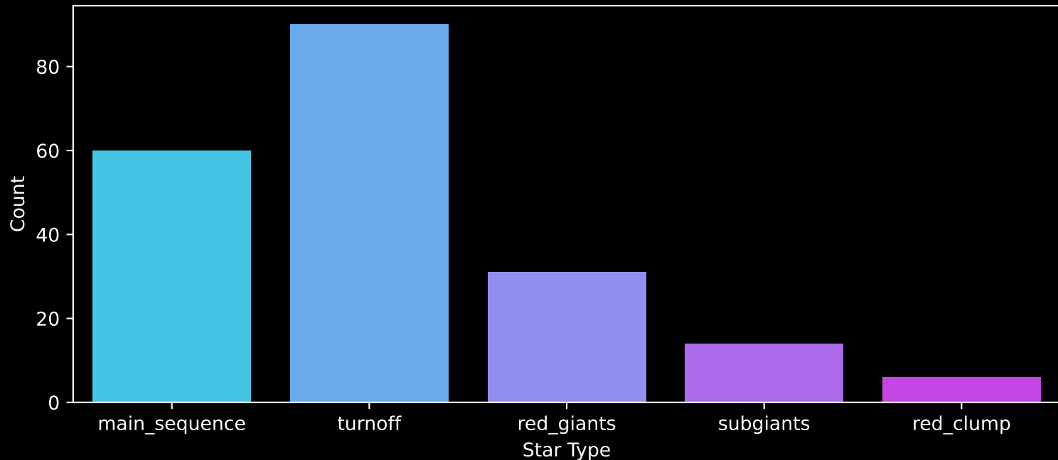
GALAH DR4 Field: [659] Count plot of Star Type
