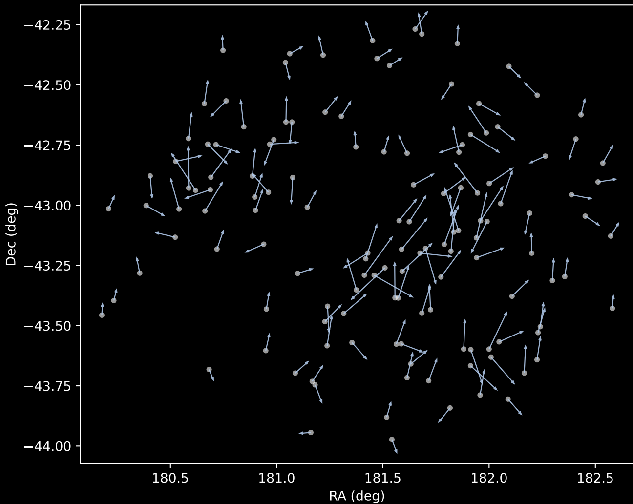
GALAH DR4 Cluster 1 Proper Motion Vectors (n=134)
