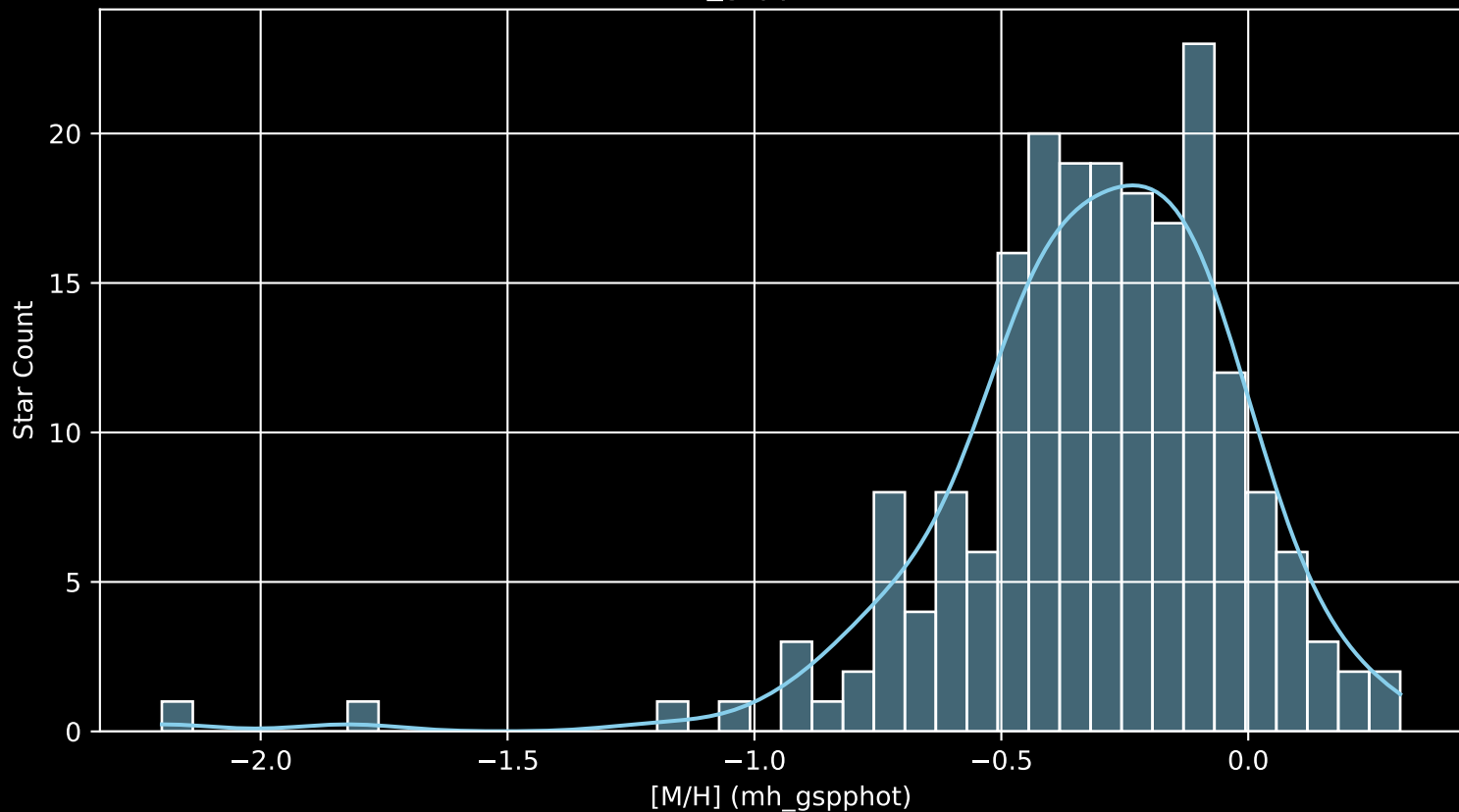
GALAH DR4 Field: [659] [M/H] (mh_gspphot) (n= 201)
